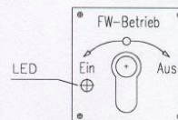
Detail FW-Schloß
